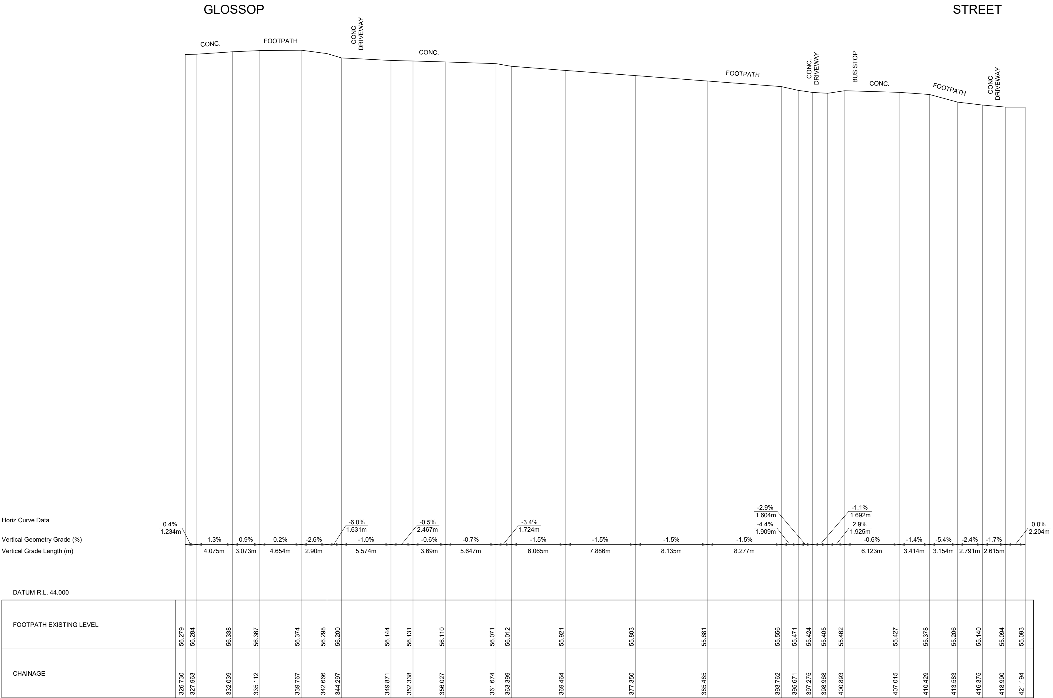
FOOTPATH LONGITUDINAL SECTION CHAINAGE 326.730 TO 421.194 HZ SCALE 1:250 & VER. SCALE 1:50
